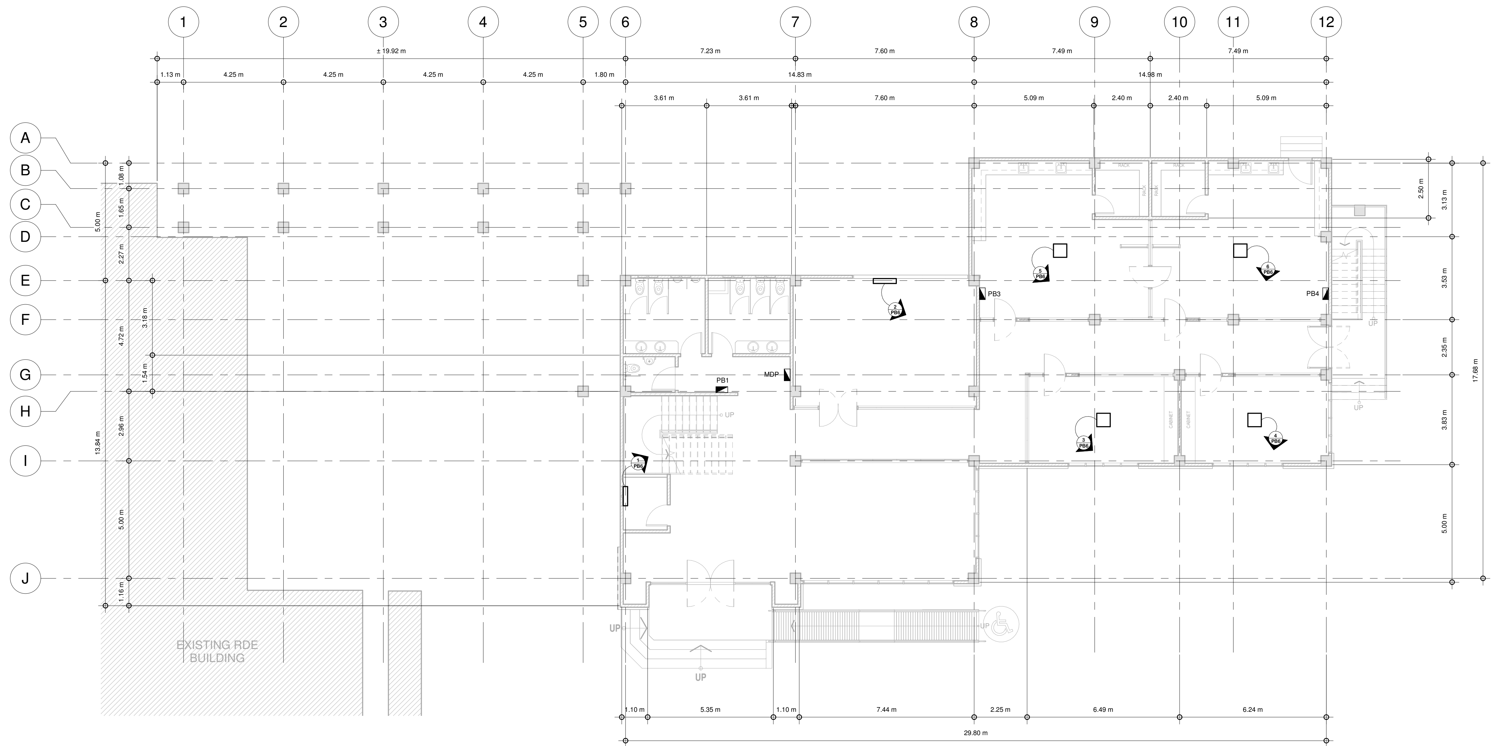
1 GROUND FLOOR ACU OUTLET LAYOUT PLAN 1 : 100 meters
